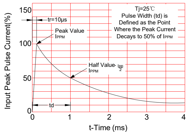
FIG.2: Pulse Waveform
