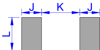
DO-214AA (SMB)
